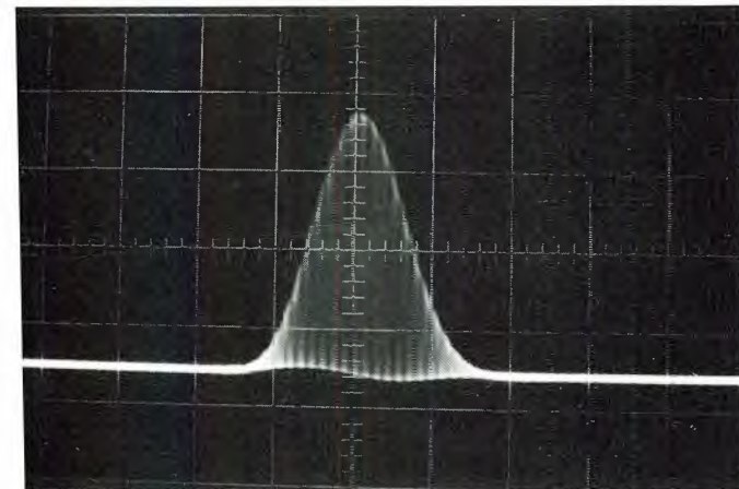
Fig. 2 Modulated 20T pulse showing 100 nanoseconds (3.58 MHz) delay.
