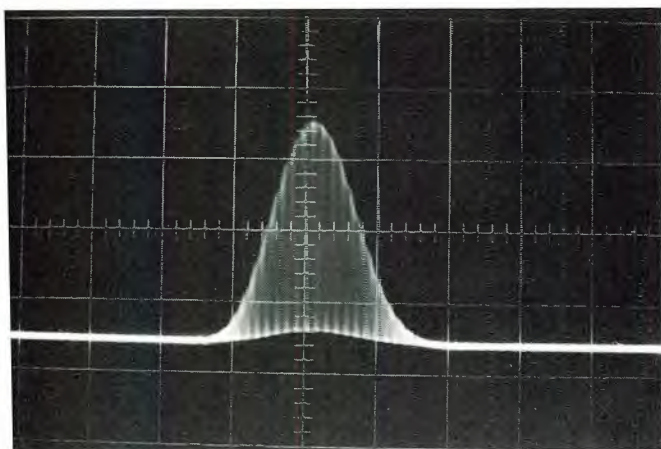
Fig. 3 Modulated 20T pulse showing 10 chrominance (3.58 MHz) attenuation.
